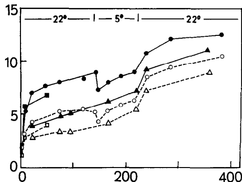
FIG. 2. The increase of the viscosity of denatured collagen solutions during the storage.
